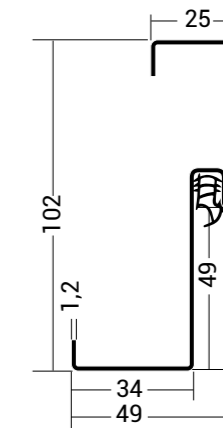
PU68 INOX STANDARD
