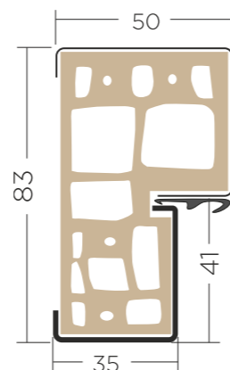
Termo ALU/PCV PU56 STANDARD
