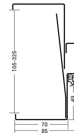
PU68-PR INOX STANDARD
